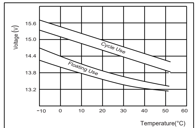
● The relationship for Charging voltage and Temperature
