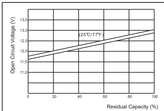
● The relationship for OCV and Capacity(25°C)
