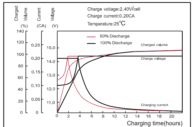
● Discharge characteristics(25°C)
