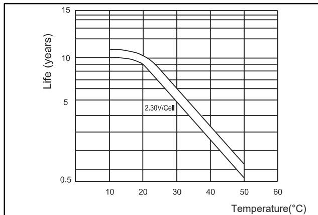
● Floating life on temperature
