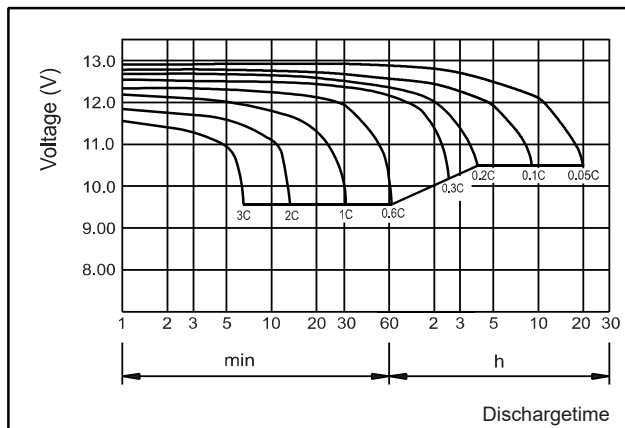
● Discharge characteristics(25°C)
