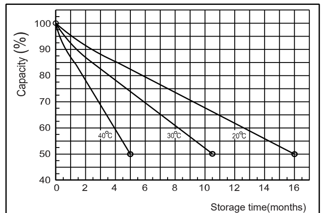
● Self-discharge characteristics
